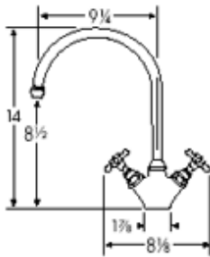
BFT-200 Series
