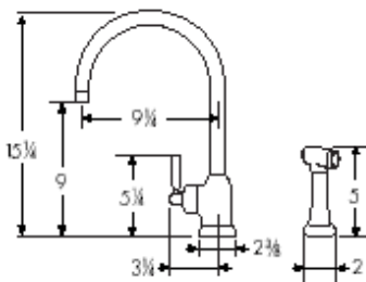
ATO-400 Series
